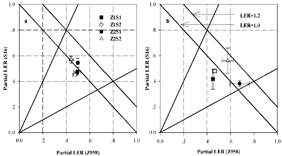
Figure 3. Partial land equivalent ratio (partial LER) of the two maize cultivars mixed planting in 2011(a) and 2012 (b). The diagonal lines show the land equivalent ratio (LER), the above area of diagonal lines of LER=1(1.2) represent there is mixing advantage according to grain yield. The two lines (the left and bottom line indicate partial LER of S16 and Z958) crossing the x - y coordinate 0-0.5 indicates a 50% to 50% balanced use of environmental sources for grains growth by S16 and Z958, values are the mean \pm SE (n=3).
