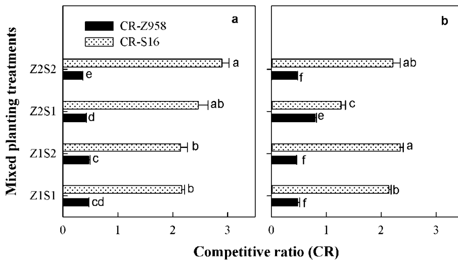
Figure 4. Competitive ratio (CR) of two maize cultivars in four mixed combinations over two years (2011, a; 2012, b), CR-Z958 showed in black bars and CR-S16 in dotted bars, the different lowercase letters in the bars means significant differences between CR z and CRs in two growing seasons, respectively.
