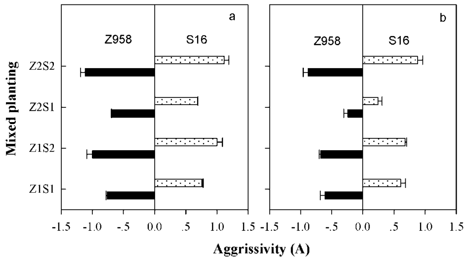
Figure 5. Aggressivity (A) between Z958 and S16 in four mixed planting patterns over two years (2011, a; 2012, b), Z958 represents as left part (black bar), S16 represents as right part (dotted bar).
