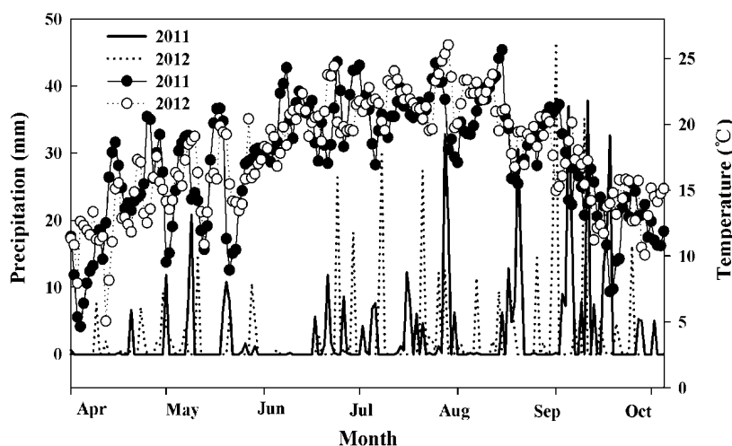
Figure 1. The daily precipitation and temperature during the two maize growing seasons, daily precipitation of 2011 (full line) and 2012 (dotted line); daily temperature of 2011 (close circle) and 2012 (open circle).
