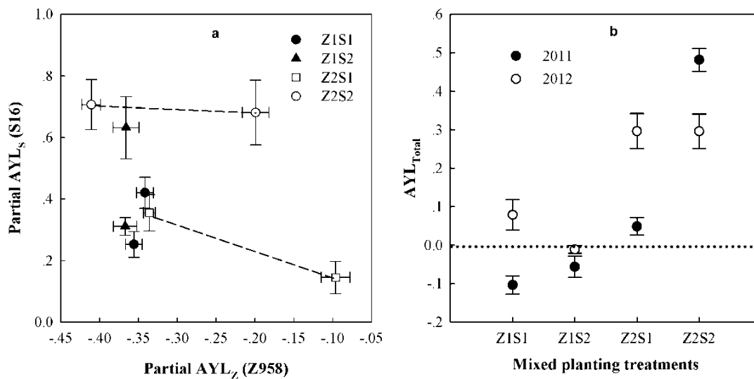
Figure 6. Partial actual yield loss (partial AYL) of two maize cultivars in four mixed combinations (a), and total AYL (AYL total , b) of that over two years, close circle, 2011; open circle, 2012. The two dash lines (a) indicated the changes of partial AYL of two maize cultivars from 2011 to 2012, the dotted line (b) means AYL total = 0, values above- and below the line mean having- or non-mixed advantage.
