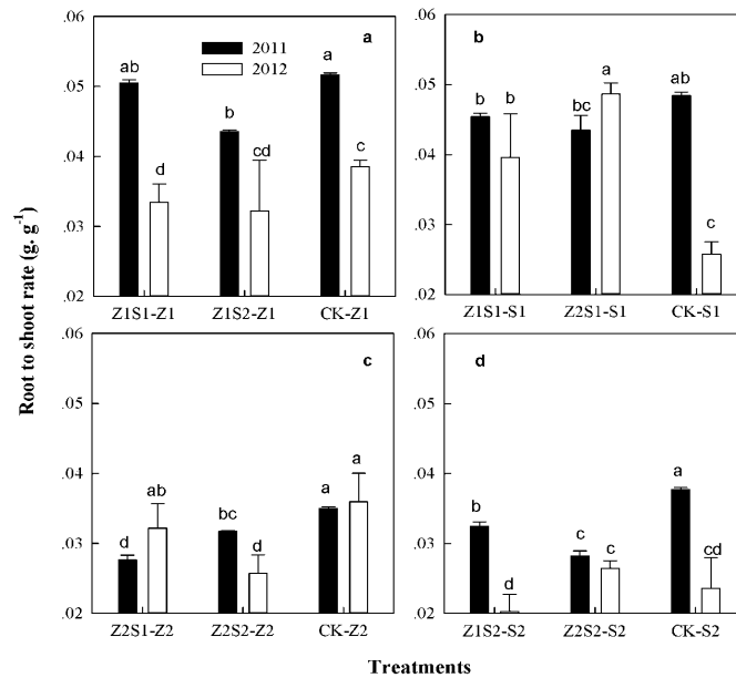
Figure 2. Root to shoot ratio between the mixed and mono-cropping treatments at harvest over two years, the data represents as 2011 (black bar) and 2012 (white bar), respectively, calculated on the basis of total dry matter of shoot and root at harvest. Different lowercase letters above the histogram bars indicated the significant differences ( P < 0.05 ) of maize cultivar under mixed and pure planting with the same density over two years.
